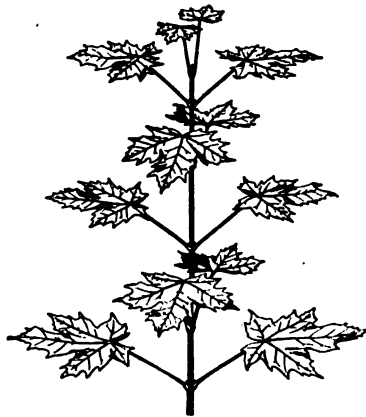
FIG. 69. — A typical leaf-bearing stem, of Norway Maple; \times \frac{1}{2} . (From Kerner.)
